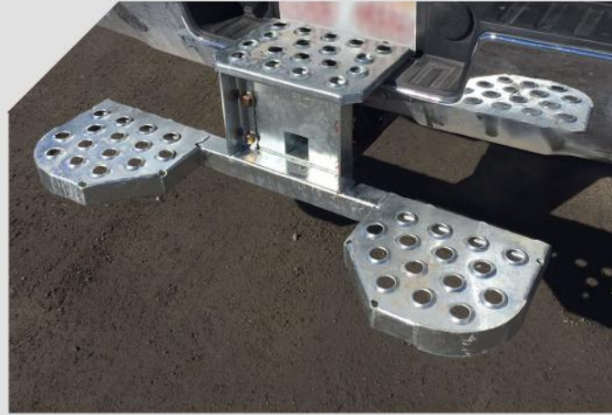
Step bumper 3 steps
